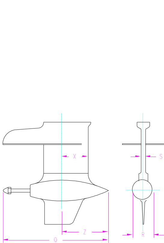
Figure 3. Lower unit
