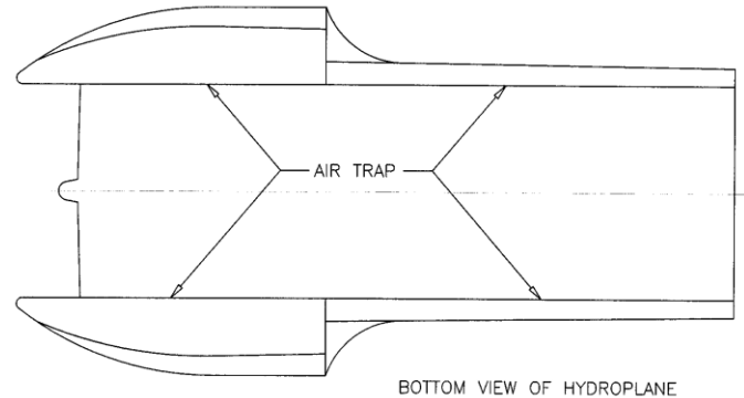
Figure 1 - Air Trap
