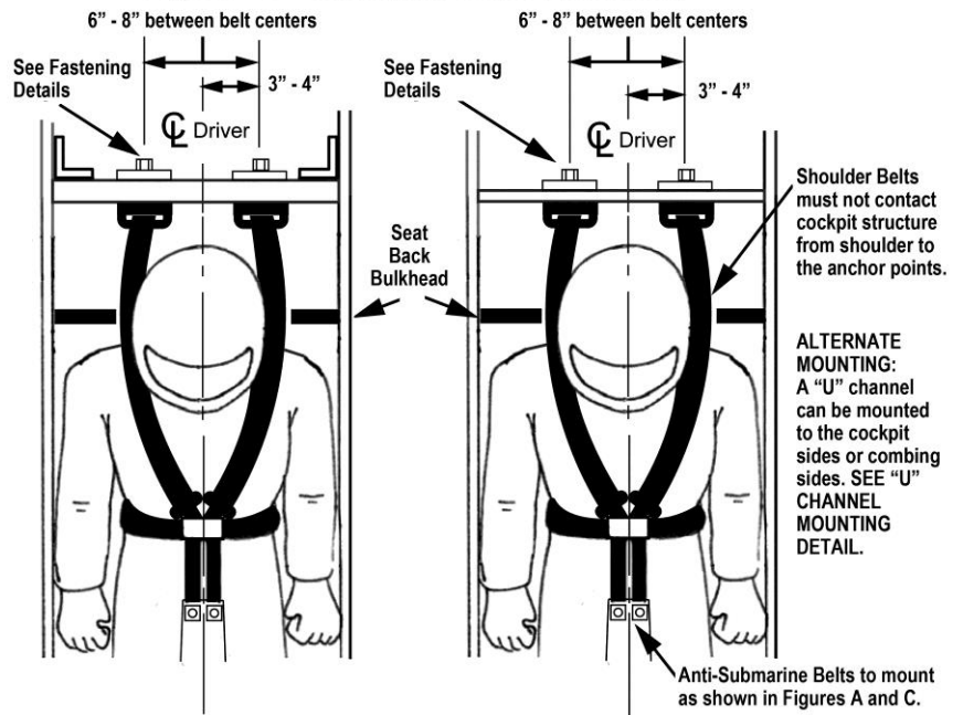
Figure "B" Shoulder Belt Anchoring
